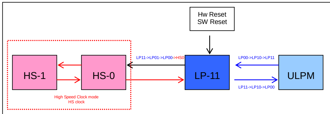
Figure 5.6: DSI Clock Lane State Diagram
